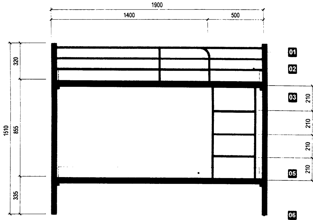
SIDE VIEW
