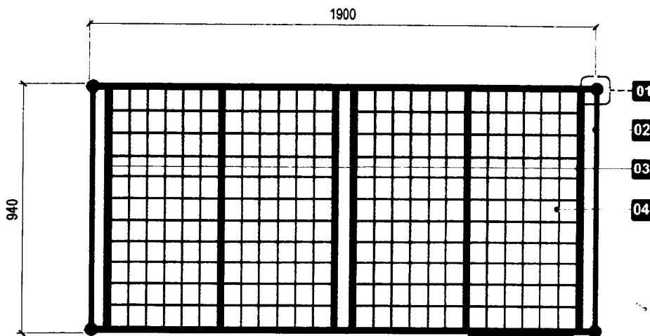
DETAILED PLAN
