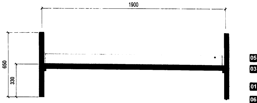
SIDE VIEW
