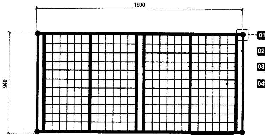
DETAILED PLAN
